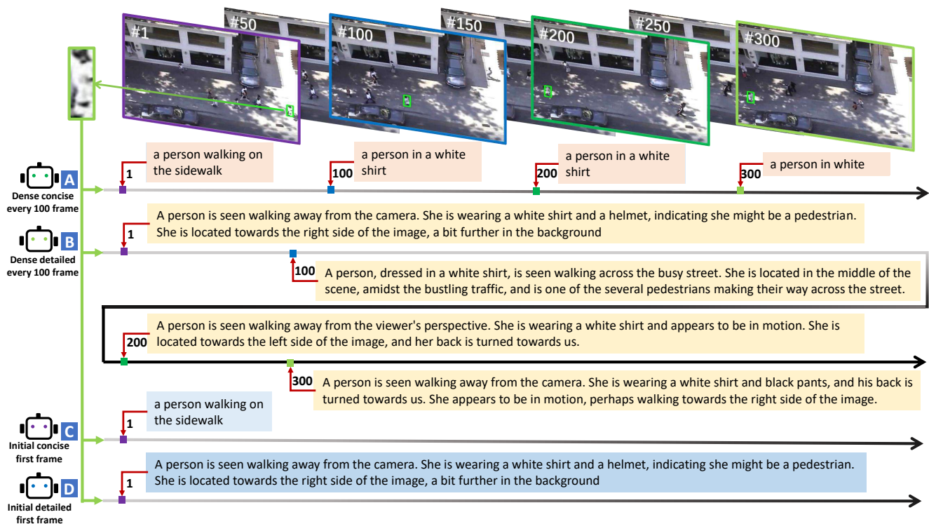
Figure 4. Examples of the four types of generated text. We provide four different natural language descriptions for each video. The object to be tracked is determined in the first frame and does not change throughout the video sequence.
